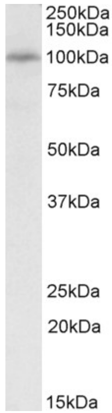
EB10087 (0.3 \mu g/ml) staining of Rat Liver lysate (35 \mu g protein in RIPA buffer). Primary incubation was 1 hour. Detected by chemiluminescence.
