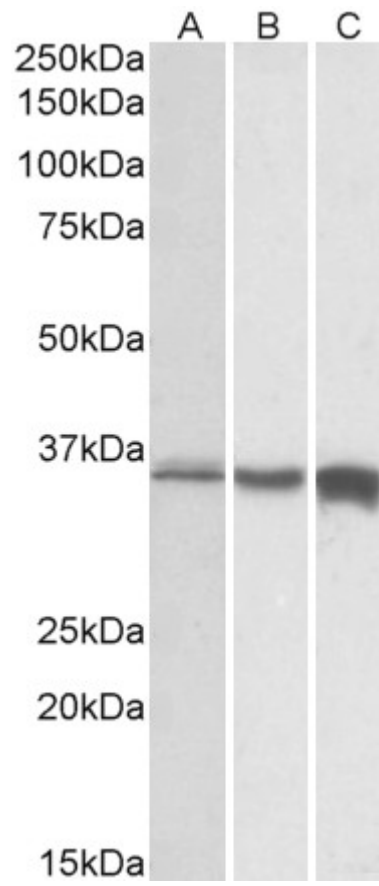
Biotinylated EB12033 (0.01 \mu g/ml) staining of Human (A), Mouse (B) and Rat (C) Skeletal Muscle lysates (35 \mu g protein in RIPA buffer). Primary incubation was 1 hour. Detected by chemiluminescence.
