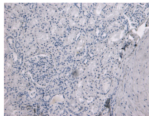
EB08219 Negative Control showing staining of paraffin embedded Human Kidney, with no primary antibody.
