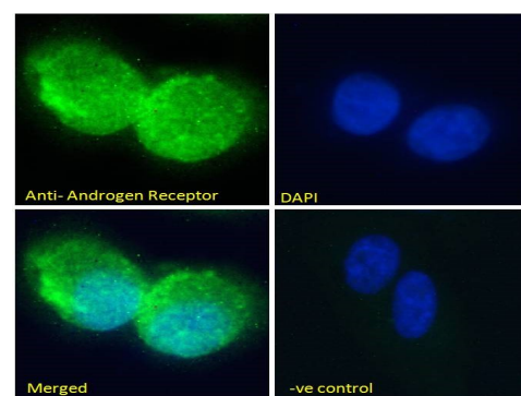
EB06441 Immunofluorescence analysis of paraformaldehyde fixed U2OS cells, permeabilized with 0.15% Triton.
