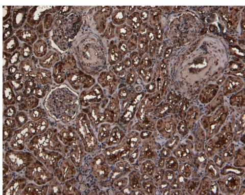
EB08219 (8µg/ml) staining of paraffin embedded Human Kidney. Heat induced antigen retrieval with citrate buffer pH 6, HRP-staining.
