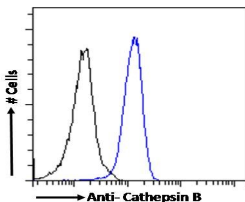
EB11975 Flow cytometric analysis of paraformaldehyde fixed HeLa cells (blue line), permeabilized with 0.5% Triton.
