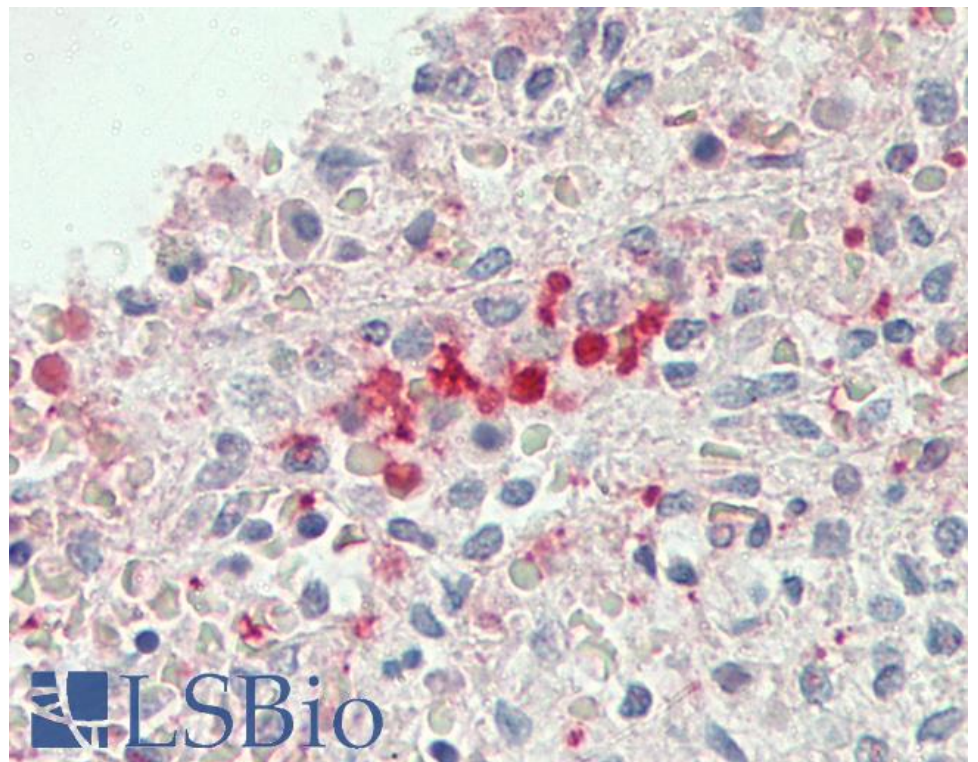
EB12401 (5µg/ml) staining of paraffin embedded Human Spleen. Steamed antigen retrieval with citrate buffer pH 6, AP-staining.
