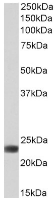
EB12401 (0.1µg/ml) staining of Human Liver lysate (35µg protein in RIPA buffer). Detected by chemiluminescence.
