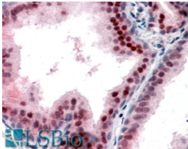
EB07131 (5µg/ml) staining of paraffin embedded Human Prostate. Steamed antigen retrieval with citrate buffer pH 6, AP-staining.
