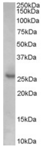
EB07131 (0.1µg/ml) staining of Human Prostate lysate (35µg protein in RIPA buffer). Detected by chemiluminescence.
