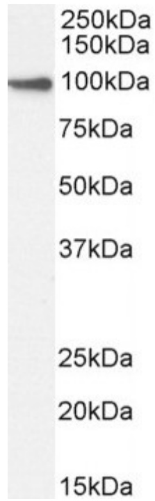
Western Blot: 1 \mu g/ml staining of Primary antibody in lysates EBL010-BMP1-S2C2, Approx.100kDa band observed (calculated MW of 111kDa according to Human NP_006120.1). Primary incubation 1 hour at room temperature. Secondary antibody is EB2ND-002-A at 1:40K
