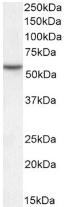
Western Blot: 0.5 \mu g/ml staining of Primary antibody in lysates EBL022-MKRN1-P1, approx.55kDa band observed. (Calculated MW of 53.3kDa according to Human NP_038474.2). Primary incubation 1 hour at room temperature. Secondary antibody is EB2ND-002-A at 1:40K.
